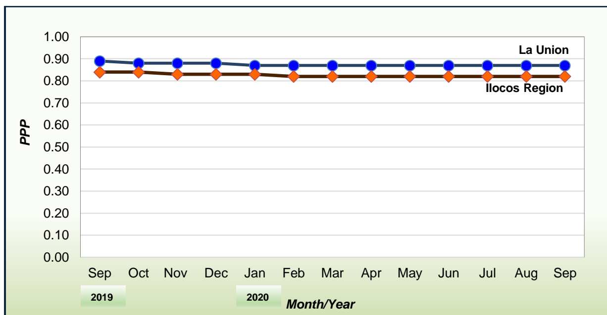
Figure 5. Purchasing Power of the Peso in La Union and Ilocos Region September 2019 – September 2020 (2012 = 100)
