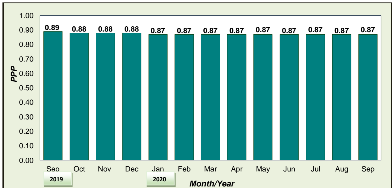
Figure 4. Purchasing Power of the Peso in La Union September 2019 – September 2020 (2012 = 100)
