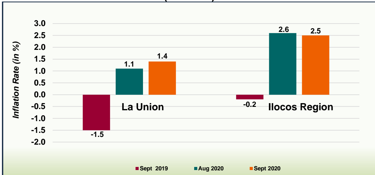
Figure 2. Headline Inflation Rates, All Items in La Union and Ilocos Region September 2019, August 2020, and September 2020 (2012=100)
