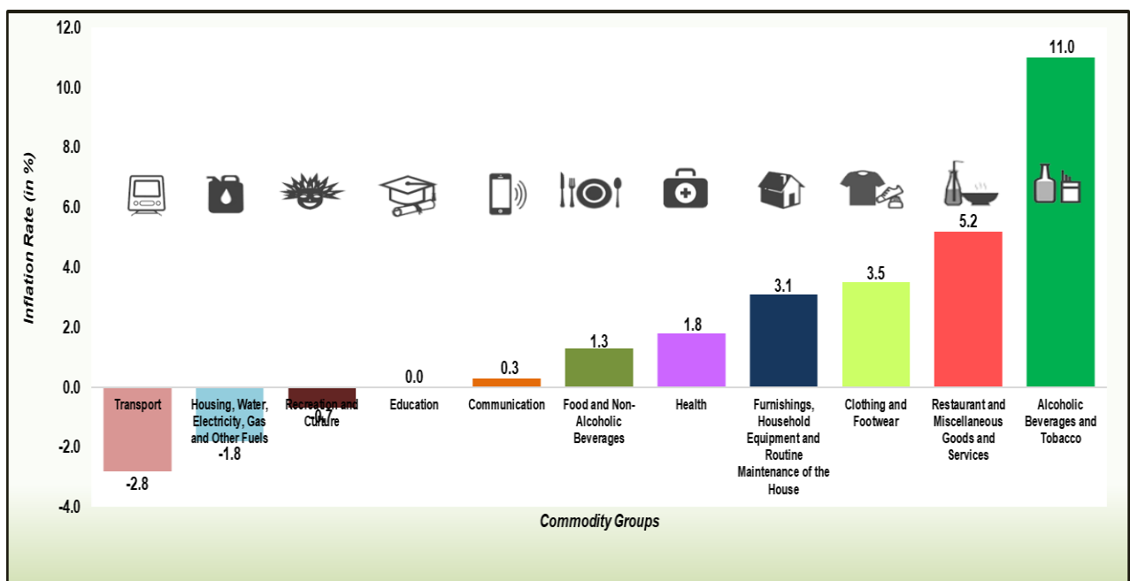
Figure 3. Inflation Rates by Commodity Groups, La Union: September 2020 (2012=100)
