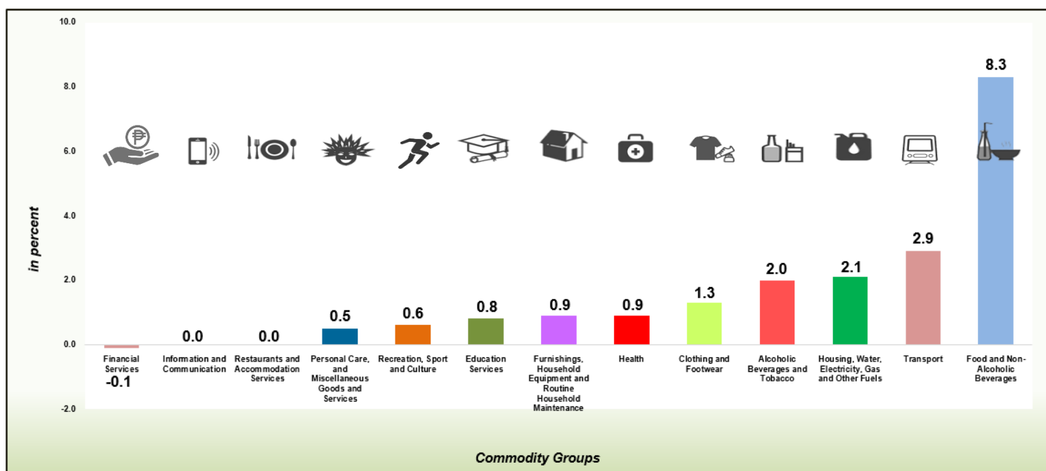
Figure 3. Inflation Rates by Commodity Groups, La Union: May 2024 (2018=100)
